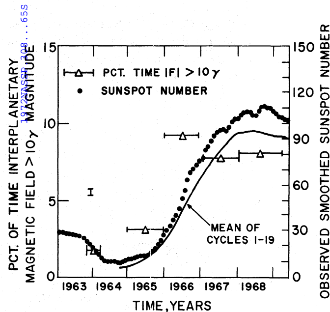
Figure 25. Percentage time the hourly average interplanetary magnetic field magnitude exceeds 10\gamma and sunspot number as a function of time in years. The enhanced field magnitudes appear to be related to enhanced sunspot number and thus possibly to solar activity. The I refers to the instantaneous field exceeding 10\gamma .
