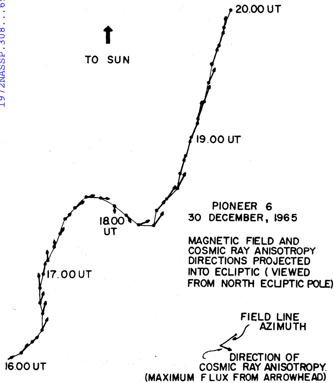
Figure 4. Interplanetary magnetic field and cosmic ray anisotropy on December 30, 1965, from Pioneer 6 observations. The interplanetary magnetic field shows a "kink" structure which is also seen in the cosmic ray anisotropy directions [McCracken and Ness, 1966].
