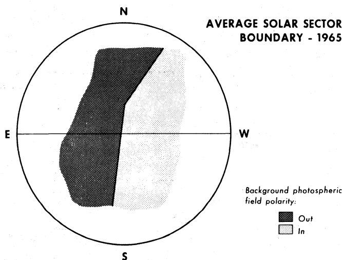
Figure 27. A schematic of Wilcox's average position of a solar sector boundary during 1965. On each side of the boundary the weak background photospheric magnetic field is predominantly of a single polarity in equatorial latitudes on both sides of the equator. This solar sector extends to latitudes near 40^\circ or 50^\circ [Wilcox, 1970b].
