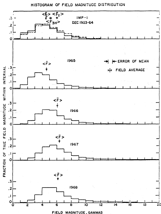
Figure 23. Interplanetary magnetic field magnitude distribution as a function of time. Average field magnitude is shown by the symbols. Somewhat different data processing has occurred throughout the years discussed in the text. Note the change from 1965 to 1966.
