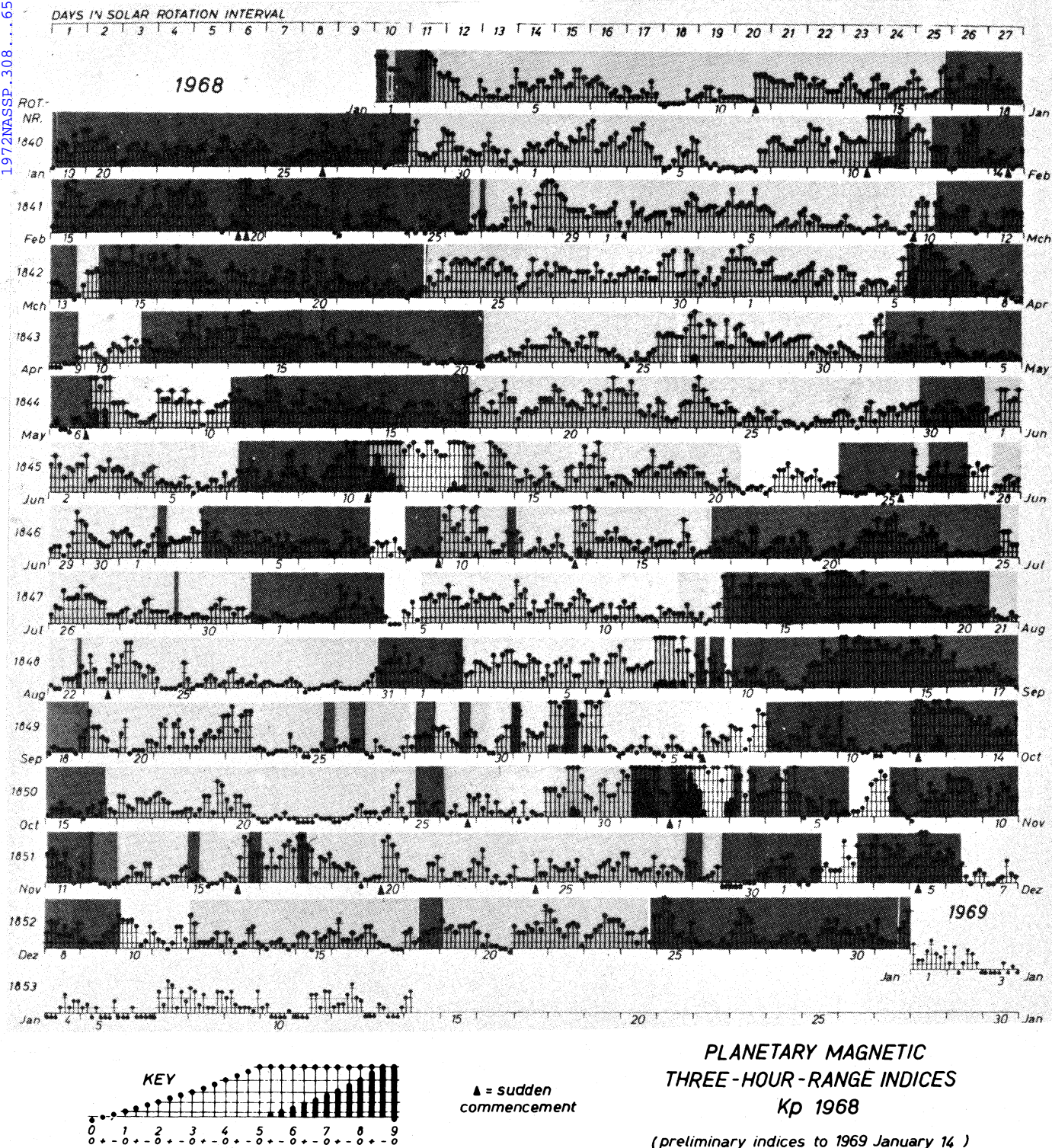
Figure 21. Interplanetary magnetic sector structure for 1968 overlaid on chart of planetary magnetic 3-hr-indices Kp [after Bartels]. The heavy shading represents magnetic field away from the sun, and the light shading, field toward the sun [Fairfield et al., 1969].
