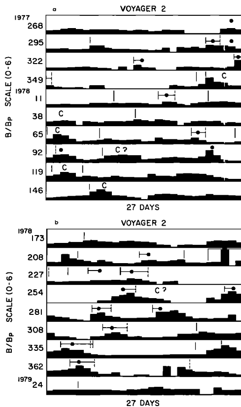
Fig. 13. Daily averages of B/B_p from Figure 7 together with the locations of shocks, interfaces and clouds from Figure 12, for both (a) the four-sector period and (b) the two-sector period.
