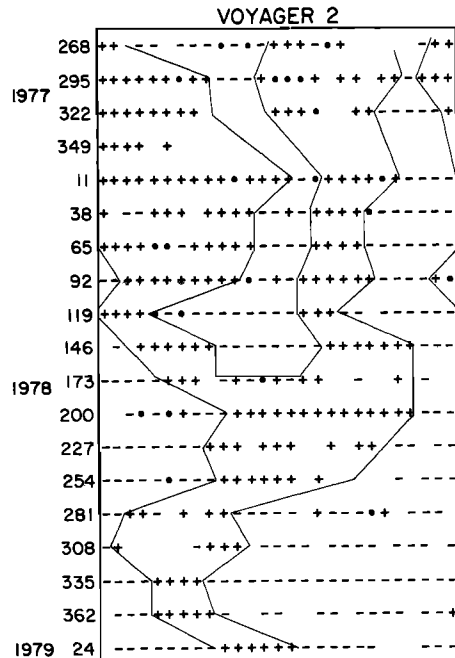
Fig. 9. Same as Figure 8, for Voyager 2 data.
