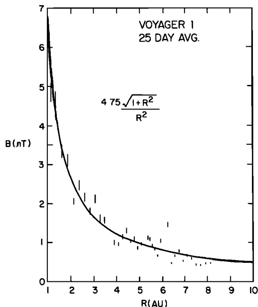
Fig. 1. Twenty-five-day averages of the interplanetary magnetic field magnitude measured by Voyager 1 as a function of radial distance from the sun. The curve is the prediction of the spiral field model with the constant A = 4.75 determined from a least squares fit to the data.
