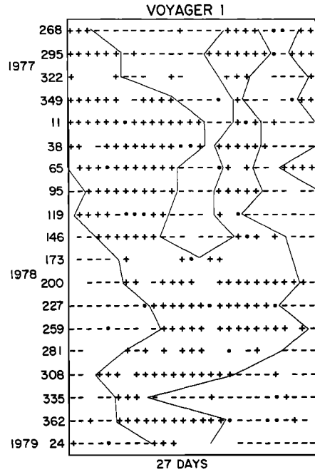
Fig. 8. The sector pattern observed by Voyager 1. Minus (plus) denotes field lines directed toward (away from) the sun, and circle denotes mixed polarity. Lines corresponding to sector boundaries are drawn to delineate the general sector pattern, but note that in many cases the appropriate position of a line is uncertain.
