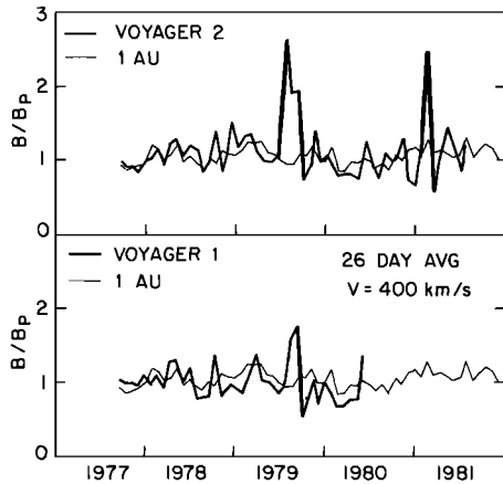
Fig. 3. Twenty-six-day averages of B/B_p , where B_p is the field strength derived from the spiral model for a given t(R) , as a function of time. Heavy lines are Voyager 1 and 2 data projected to 1 AU assuming a time delay appropriate for corotating flows with a constant solar wind speed of 400 km/s. The light line is the field strength observed at 1 AU, with B_p = 6.7 nT; it was derived from IMP 8 and ISEE 3 data. No significant systematic differences are observed between the Voyager data obtained at large distances from the sun and the 1 AU data.
