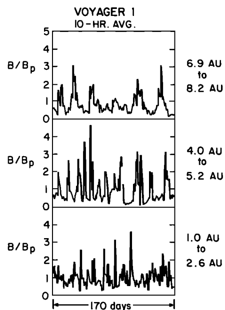
Fig. 4. Examples of the large-scale fluctuations in B/B_p observed by Voyager 1 at three different distances from the sun; 10-hour averages of B/B_p are plotted.
