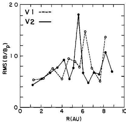
Fig. 5. The rms of B/B_p computed for successive 100-day intervals, plotted as a function of radial distance from the sun. Each point is the average distance of the spacecraft in the corresponding 100-day interval.
