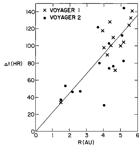
Fig. 14. The time interval between the arrival of a forward shock and a corresponding reverse shock for shock pairs identified by Voyager 1 and 2 plotted as a function of the distance at which the shock pair was observed.
