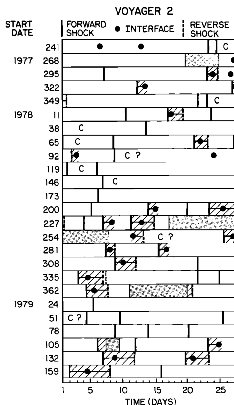
Fig. 12. The same as Figure 11, except that the results are for Voyager 2.
