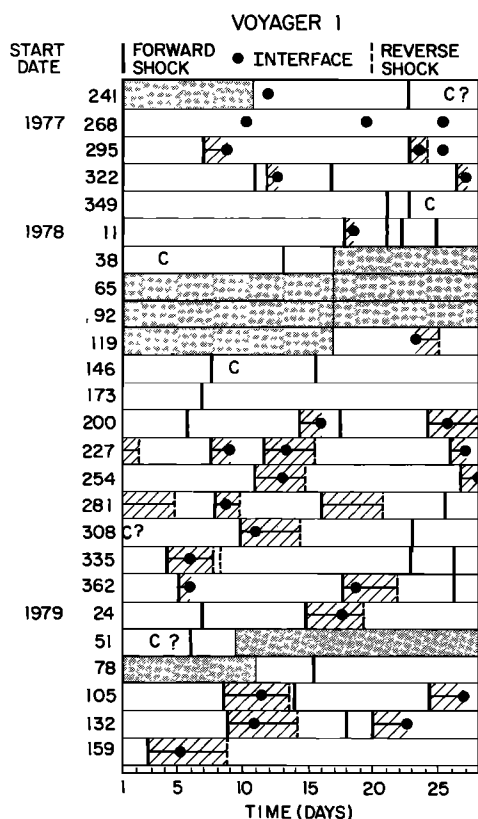
Fig. 11. This shows the temporal locations of forward shocks (solid lines), reverse shocks (dashed lines), interfaces (solid dots) and magnetic clouds (denoted by C) identified using hour averages of plasma and magnetic field data from Voyager 1. Shaded areas indicate data gaps.
