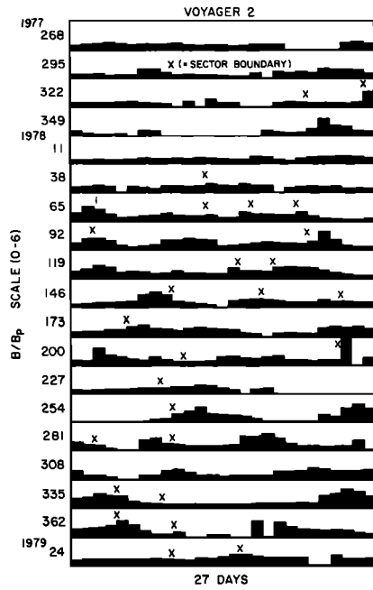
Fig. 7. Daily averages of B/B_p determined from Voyager 2 data plotted in successive 27-day intervals. The crosses represent the positions of well-defined sector boundaries (see Figure 9).
