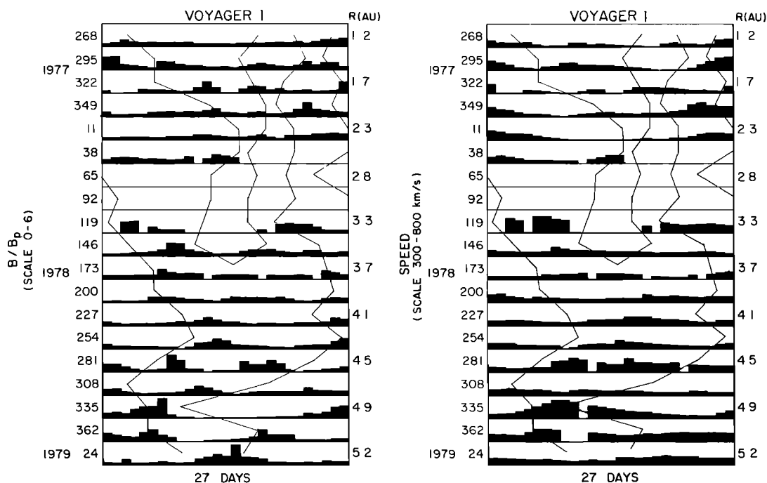
Fig. 10. Left: The sector pattern from Figure 8 superimposed on a plot of daily averages of B/B_p from Voyager 1 data. Right: The sector pattern from Figure 8 superimposed on a plot of daily averages of the bulk speed measured by Voyager 1.
