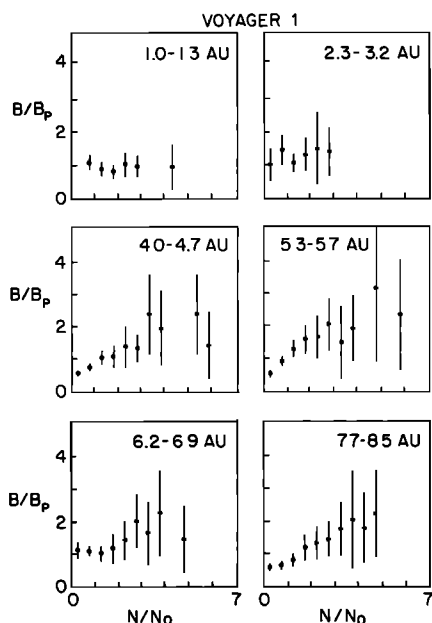
Fig. 15. B/B_p versus N/N_p , where N is the plasma density, and N_p = 6 (R(\text{AU}))^{-2} for six different distance intervals.
