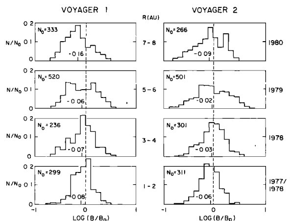
Fig. 6. Distributions of 10-hour averages of B/B_p at different distances from Voyager 1 and 2 data.
