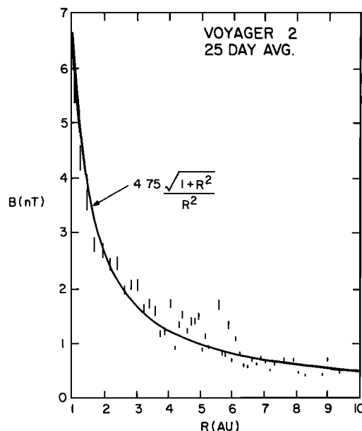
Fig. 2. Same as Figure 1, except that Voyager 2 data are plotted.
